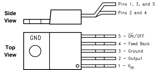
Figure 1. Bent and Staggered Leads, Through Hole Package 5-Lead TO-220 (T)
