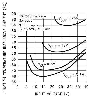
Figure 20. Junction Temperature Rise, TO-263
