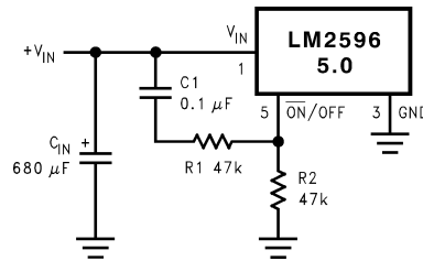
Figure 21. Delayed Startup
