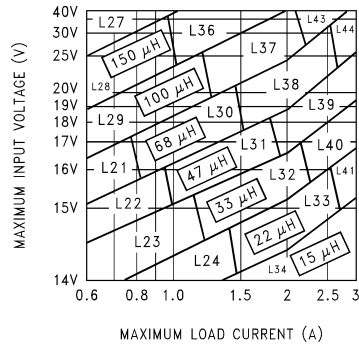
Figure 11. LM2596-12
