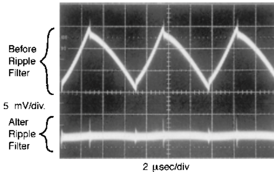
Figure 17. Post Ripple Filter Waveform
