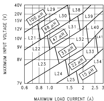
Figure 10. LM2596-5.0
