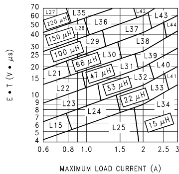
Figure 12. LM2596-ADJ
