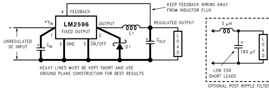
Figure 7. Fixed Output Voltage Versions
