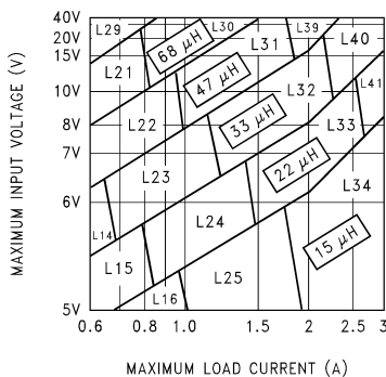
Figure 9. LM2596-3.3
