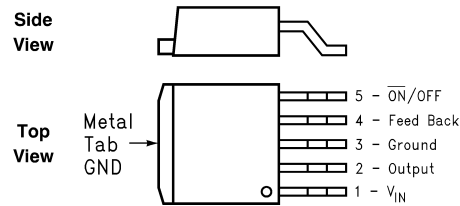
Figure 2. Surface Mount Package 5-Lead TO-263 (S)
